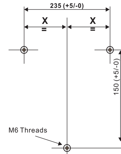
MOUNTING DETAILS
